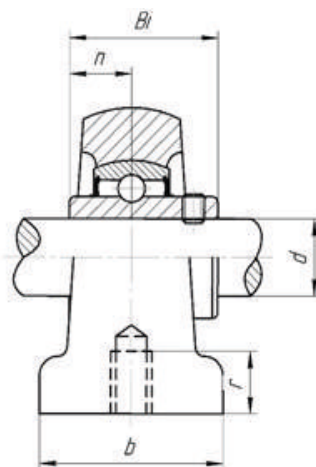
MOUNTED BEARING UNIT USPA200 SERIES PILLOW BLOCK
